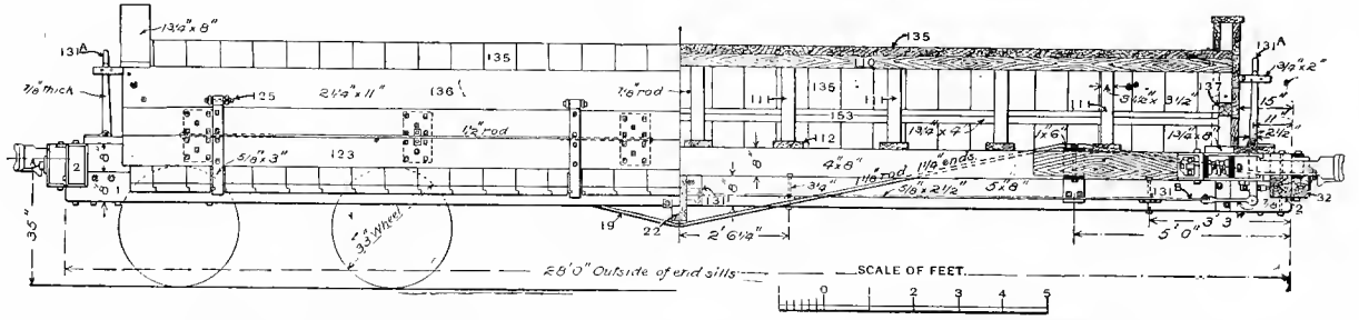
Fig. 328. Half Side Elevation. Half Longitudinal Section.
